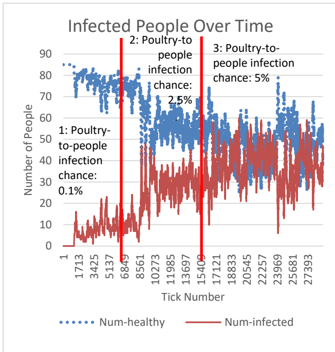
Figure 4: Number of infected people over time with different poultry-to-people infection changes
