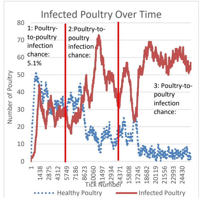
Figure 5: Number of infected poultry over time with different poultry-to-poultry infection chances
