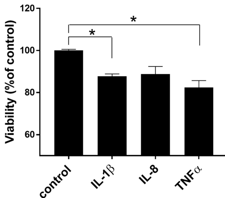
Figure 6. Effect of human recombinant IL-1 \beta , IL-8, and TNF \alpha on hFOB cell viability MTT assay results from hFOB cells treated with human recombinant IL-1 \beta (100 ng/mL), IL-8 (100 ng/mL), and TNF \alpha (10 ng/mL) for 24 h. Significance was determined using a student t -test with p -value < 0.05. * indicates a significant difference between treated groups and the control.
