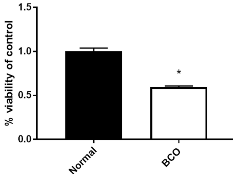
Figure 1. Effect of plasma from normal and BCO-affected broilers on hFOB cell viability. MTT assay results from hFOB cells treated with media containing 5% plasma from either normal (non-lame and no lesions of the bone) or BCO-affected (lame with lesions in both legs) broilers for 4 h. Significance was determined using a student t -test with p -value < 0.05 . * indicates a significant difference between groups.
