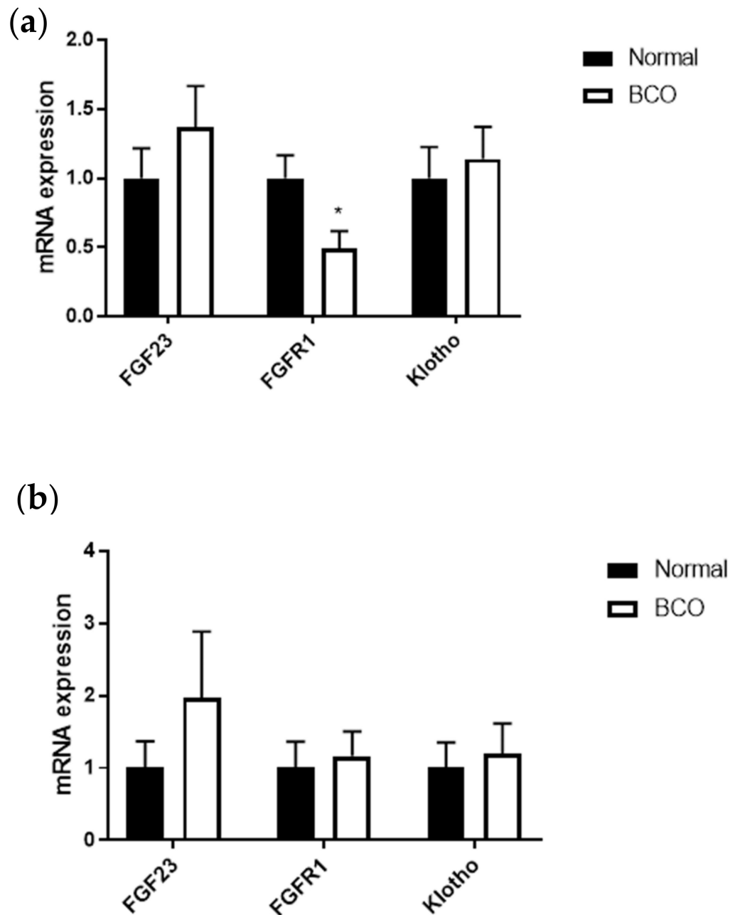
Figure 5. Local and systemic expression of key FGFs in normal and BCO-affected broilers. Gene expression for FGF23 , FGFR1 , and Klotho in the bone (a) and blood (b) of normal and BCO-affected broiler chickens. Significance was determined using a student t -test with p -value < 0.05. * indicates a significant difference between normal and BCO.
