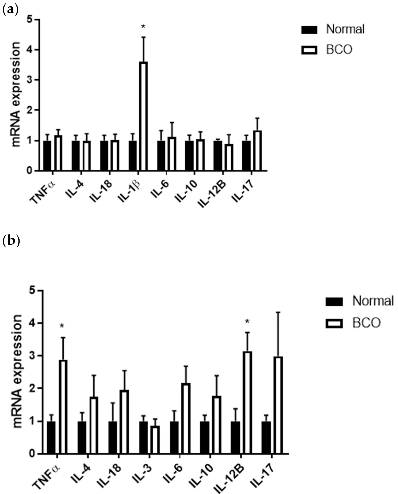
Figure 2. Local and systemic cytokine profile in normal and BCO-affected broilers. Gene expression for TNF \alpha , IL-4 , IL-18 , IL-1 \beta , IL-6 , IL-10 , IL-12B , IL-17 , and IL-3 in bone (a) and blood (b) of normal and BCO-affected broiler chickens. Significance was determined using a student t -test with p -value < 0.05. * indicates significant difference between normal and BCO.
