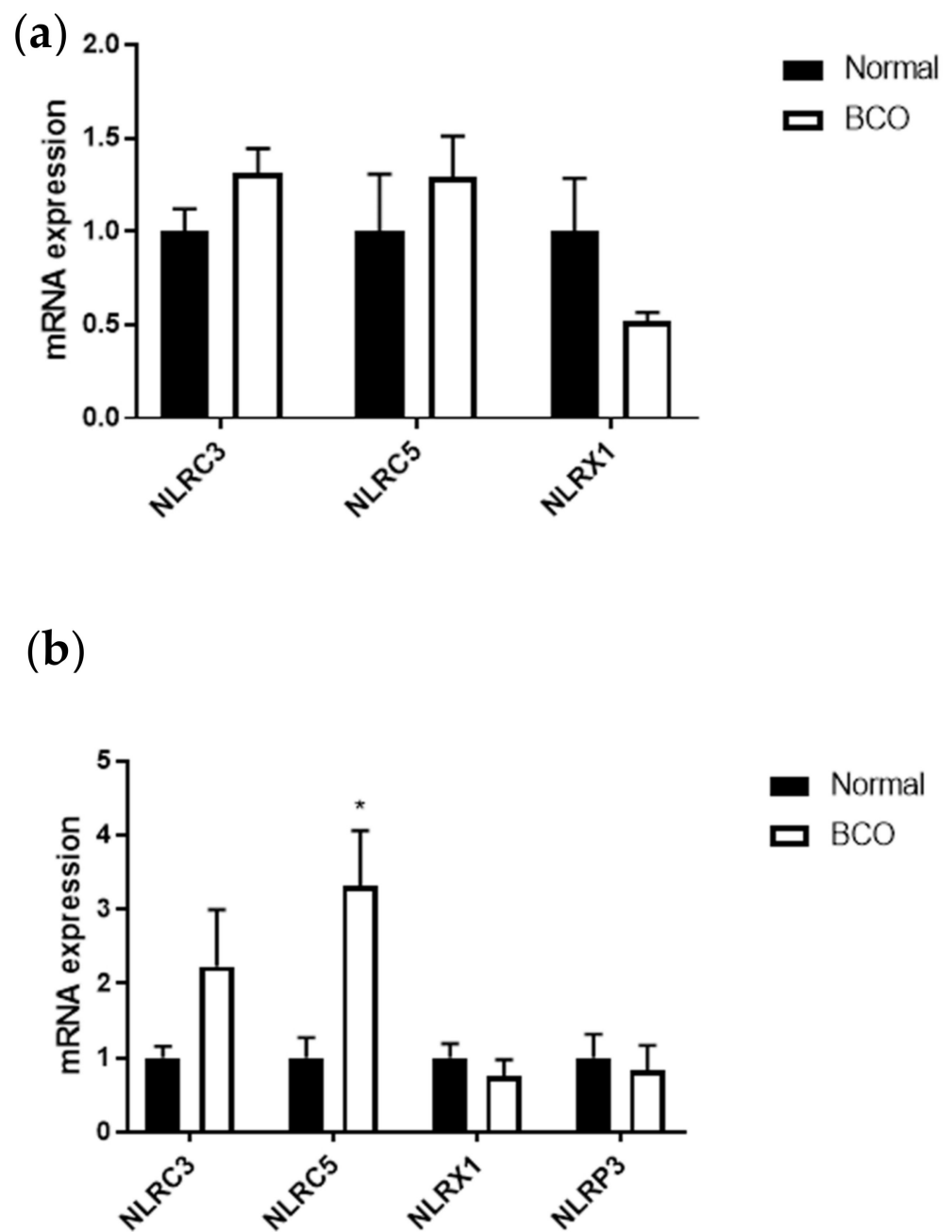
Figure 4. Local and systemic inflammasome profile in normal and BCO-affected broilers. Gene expression for NLRC3 , NLRC5 , and NLRX1 in bone (a) and blood (b) of normal and BCO-affected broiler chickens, as well as the expression of NLRP3 in blood (b). Significance was determined using a student t -test with p -value < 0.05. * indicates a significant difference between normal and BCO.
