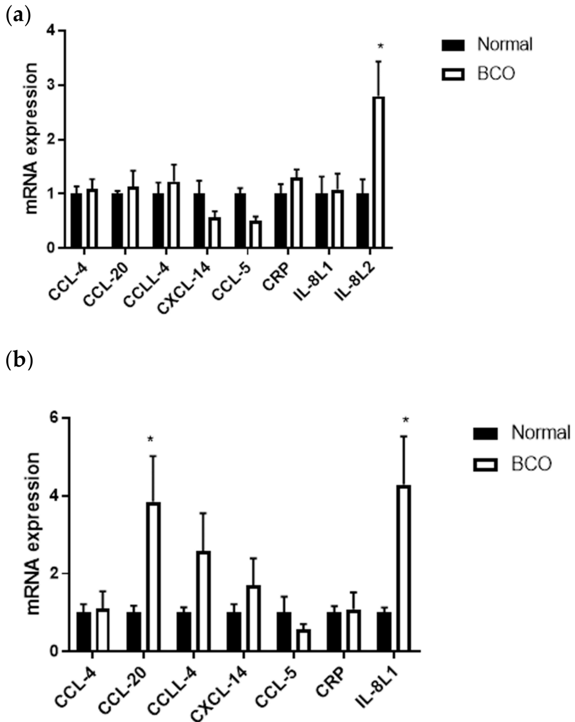
Figure 3. Local and systemic chemokine profile in normal and BCO-affected broilers. Gene expression for CCL-4 , CCL-20 , CCLL-4 , CXCL-14 , CCL-5 , CRP , and IL-8L1/IL-8L2 in bone (a) and blood (b) of normal and BCO-affected broiler chickens. Significance was determined using a student t -test with p -value < 0.05. * indicates significant difference between normal and BCO.
