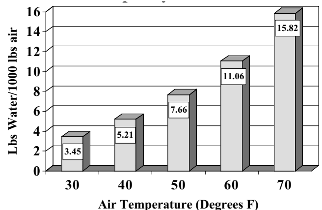
Figure 1. Moisture Holding Capacity of Air
