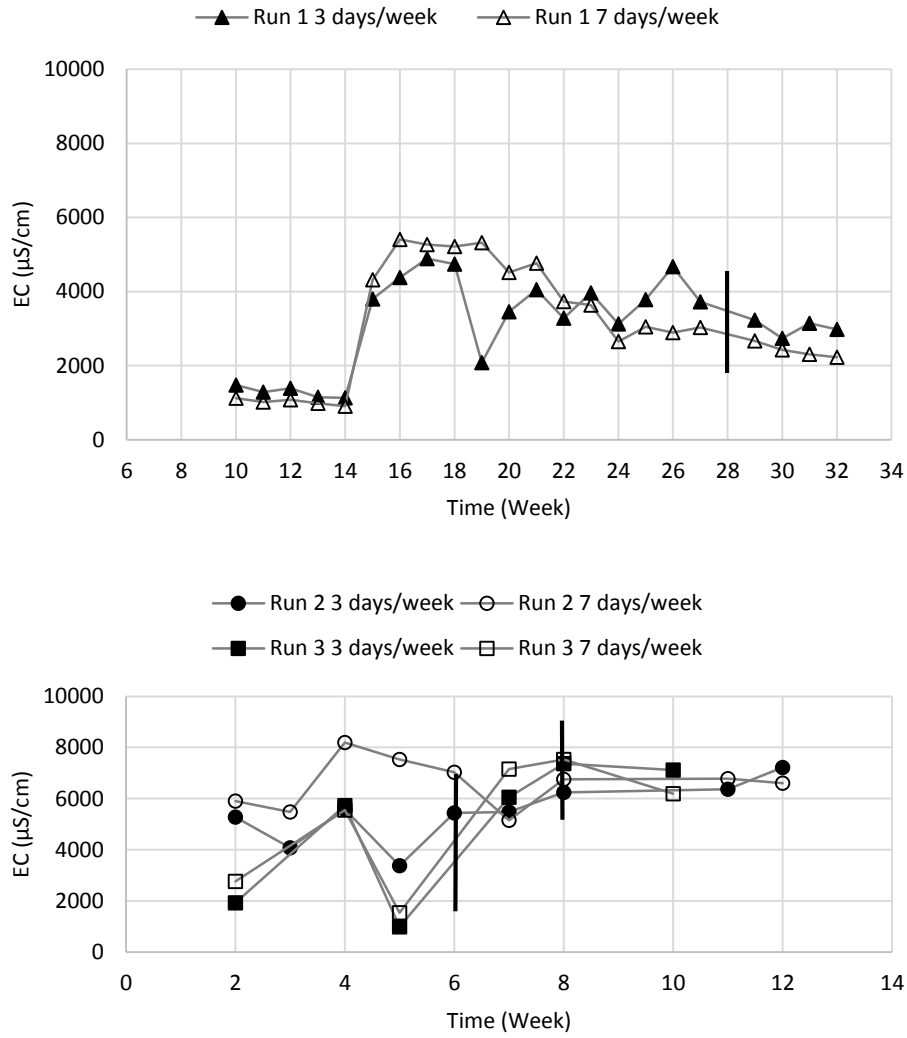
Figure 2. Average electrical conductivity for runs 1, 2, and 3. Solid lines at weeks 28, 8, and 6 indicate the beginning of the 30-day composting period for runs 1, 2, and 3, respectively.
