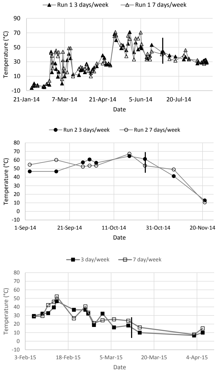
Figure 1. Temperatures for runs 1, 2, and 3. Solid lines indicate the beginning of the 30-day composting period for each run.
