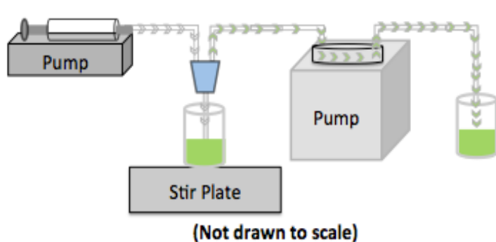
Figure 4. Push-pull schematic.
