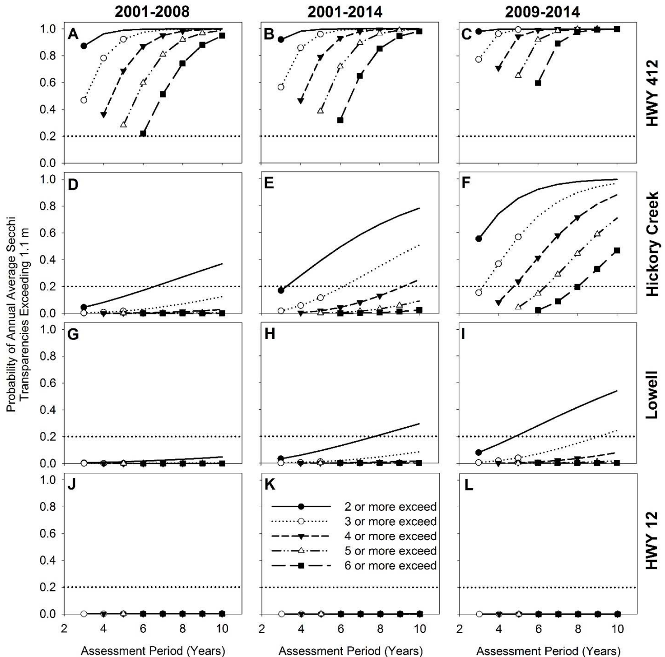
Figure 6. Probability of exceeding the 1.1 m average annual Secchi transparency (ST) standard where the number of exceedances is varied across a variable assessment period for A) Highway 412 using 2001-2008 data, B) Highway 412 using 2001-2014 data, C) Highway 412 using 2009-2014 data, D) Hickory Creek using 2001-2008 data, E) Hickory Creek using 2001-2014 data, F) Hickory Creek using 2009-2014 data, G) Lowell using 2001-2008 data, H) Lowell using 2001-2014 data, I) Lowell using 2009-2014 data, J) Highway 12 using 2001-2008 data, K) Highway 12 using 2001-2014 data, L) Highway 412 using 2009-2014 data.
