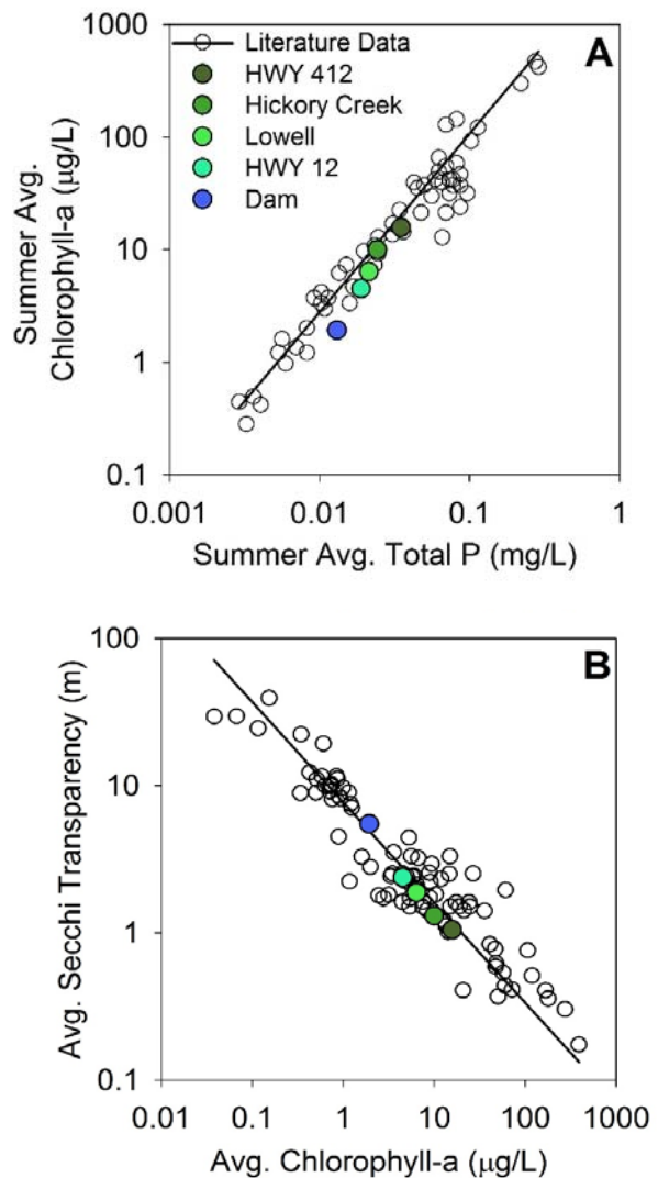
Figure 2. A) Relationship between average summer total P concentration and average summer chlorophyll a (chl-a) concentration in lakes from Dillon and Rigler (1974) along with data from each location on Beaver Lake, B) Relationship between average summer chl-a concentration and average summer Secchi transparency (ST) from Carlson (1977) along with data from each location on Beaver Lake.
