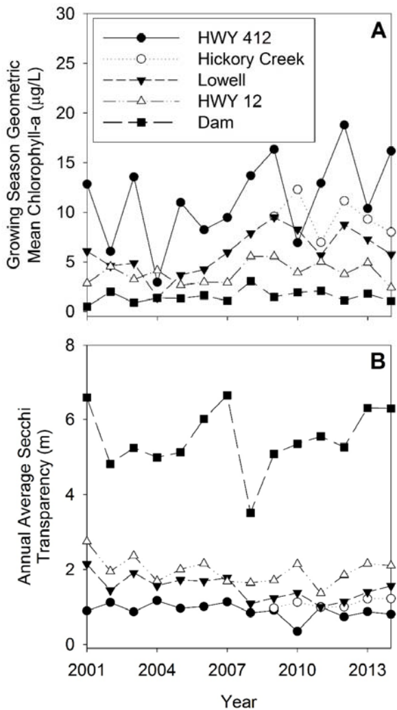
Figure 3. Long-term trends in A) growing season geometric mean chlorophyll a (chl-a) concentrations, and B) annual average Secchi transparencies (ST) at sites in Beaver Lake.
