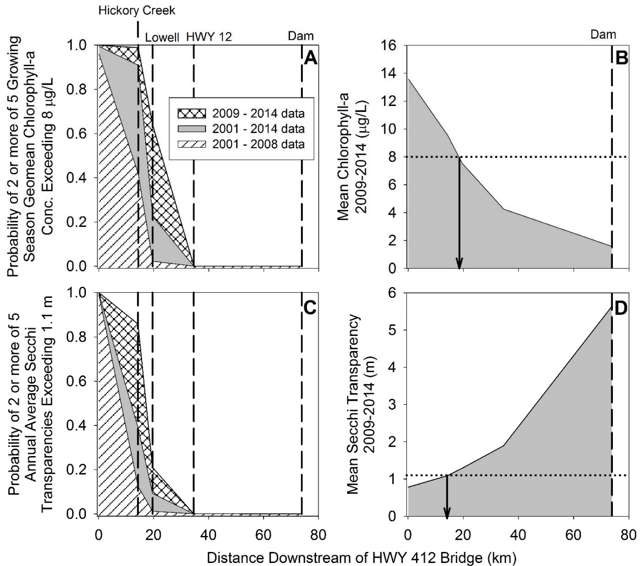
Figure 4. Probability of exceeding the water quality standards for A) chlorophyll a (chl-a) and C) Secchi transparency (ST) using data collected before 2009 and data from the entire period of record; and the mean of observed values from 2009-2014 for B) chl-a and D) ST along the riverine-transition-lacustrine gradient in Beaver Lake.
