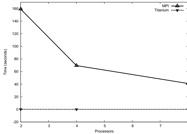
Figure 21: SM Transform - 2048x2048 Matrix
