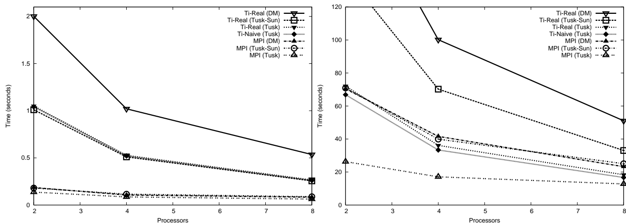
Figure 15: Tusk/Tusk-Sun Comparison Runs - Multiply with length 256 Figure 16: Tusk/Tusk-Sun Comparison Runs - Multiply Matrix 1024
