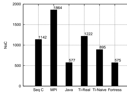
Figure 30: NoC Multiply
