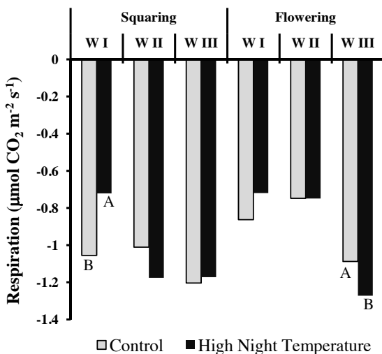
Fig. 1. Effect of high night temperature on respiration one (W I), two (W II) and three (W III) weeks after the night temperature was raised. Control night temperature = 24 °C and high night temperature = 29 °C. Columns with different letters within a growth stage are significantly different ( P = 0.05 ). LSD squaring 0.25 (0.02); LSD flowering 0.19 (0.05).
