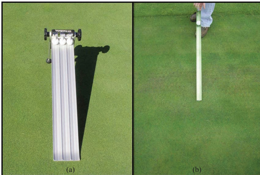
Fig. 1. Turf researchers using the Pelzmeter (a) and the Stimpmeter (b) to measure putting green speed.
