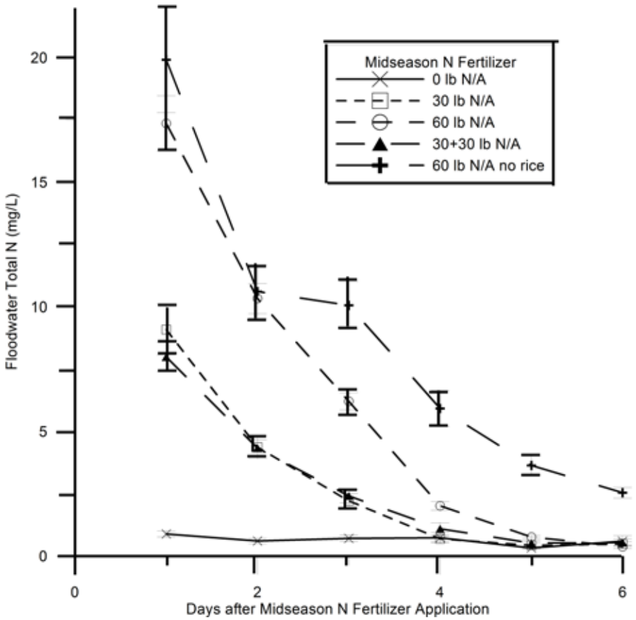
Fig. 6. Floodwater total N concentrations for each treatment of the midseason N fertilizer application with standard error bars at \alpha=0.05 .
