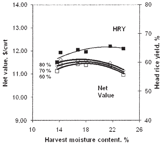
Fig. 3. Net value (eq. 5) and head rice yield (HRY) (■) of Cypress rice harvested from Stuttgart, Ark., in 2000. Net value was calculated assuming that head rice had a value of $18.00/cwt, and brokens had values of 60 (□), 70 (x), or 80% (◇) of the head rice value. Drying charges were calculated per equation 1 using the drying fee structure detailed in Table 2.
