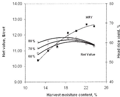
Fig. 2. Net value (eq. 5) and head rice yield (HRY) (■) of Bengal rice harvested from Stuttgart, Ark., in 2000. Net value was calculated assuming that head rice had a value of $18.00/cwt, and brokens had values of 60 (□), 70 (x), or 80% (◇) of the head rice value. Drying charges were calculated per equation 1 using the drying fee structure detailed in Table 2.
