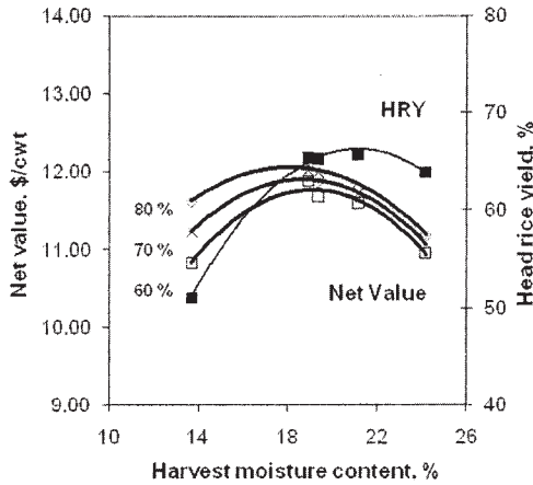
Fig. 1. Net value (eq. 5) and head rice yield (HRY) (■) of Wells rice harvested from Osceola, Ark., in 2006. Net value was calculated assuming that head rice had a value of $18.00/cwt, and brokens had values of 60 (□), 70 (x), or 80% (◇) of the head rice value. Drying charges were calculated per equation 1 using the drying fee structure detailed in Table 2.
