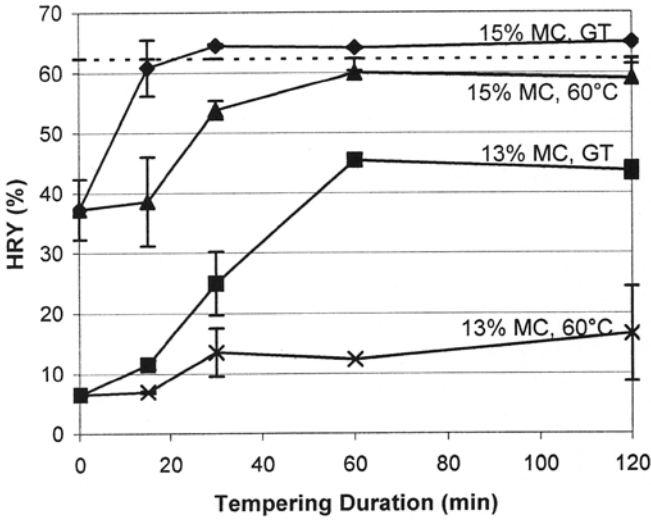
Fig. 1. Head rice yield (HRY) data of Wells [21.9% initial moisture content (MC)] dried at 120°C, ~1.3% RH to 13% or 15% moisture content (MC) and tempered at the grain temperature (GT) or 60°C for various durations. The dotted line represents the control HRY of 62.3%. Vertical bars display standard deviation from the mean of two replications.
