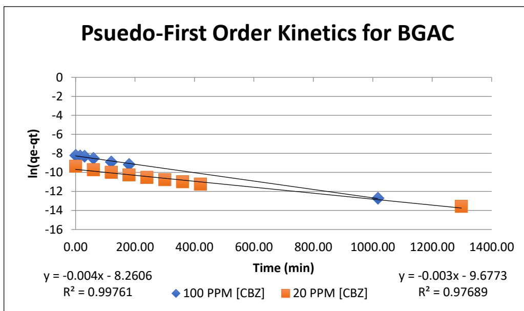
Figure 7.2.4: Pseudo-First Order Kinetics of a 20 ppm and 100 ppm Carbamazepine BGAC solution, with proportional concentrations of sucrose.
