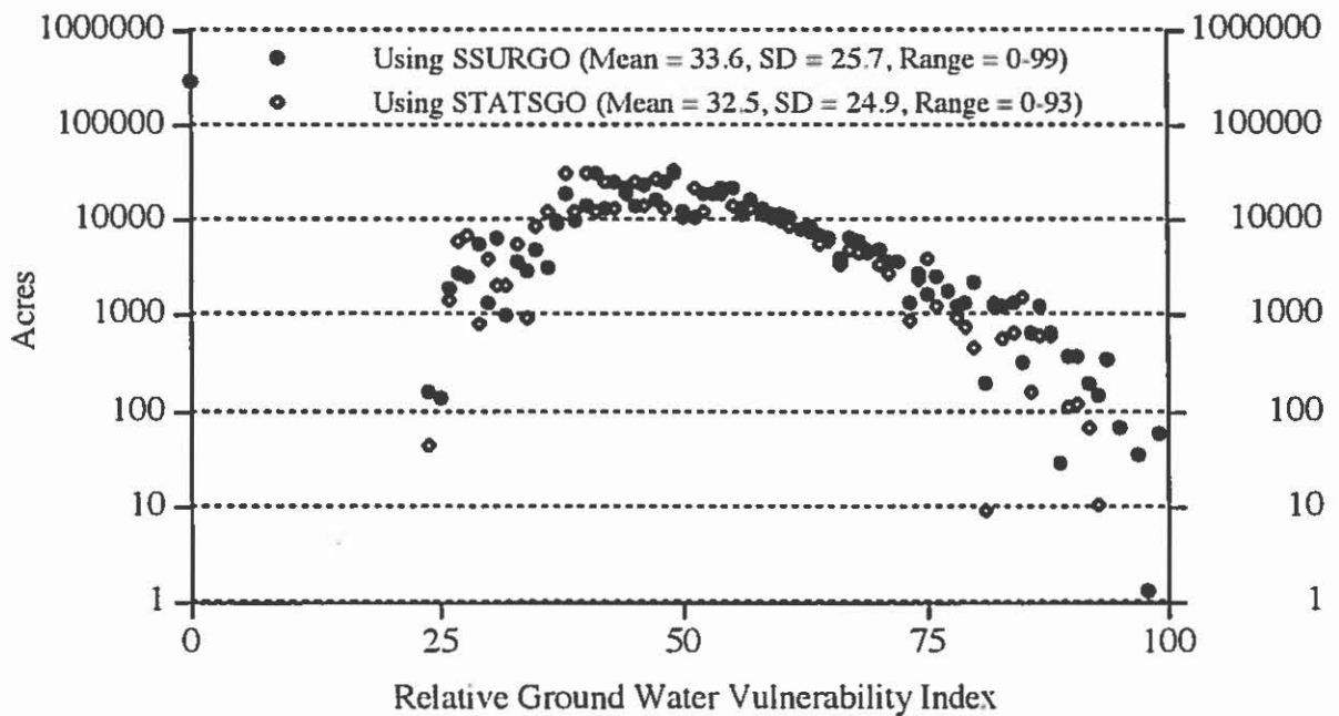
Fig. 14 Comparison of ground water vulnerability index in Lonoke & Prairie counties using SSURGO vs. STATSGO input soil maps
