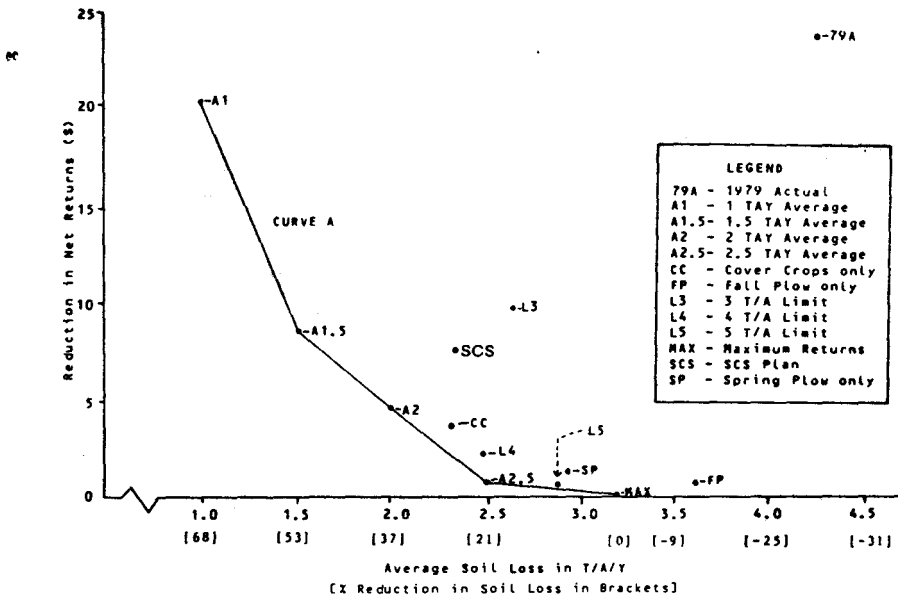
Fig. 3. Relationship between Soil Loss and Reduction in Net Returns
