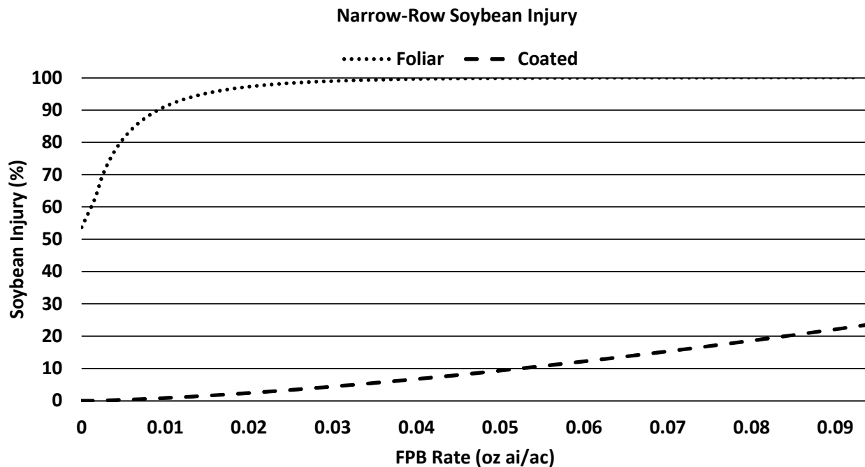
Fig. 2. Weibull growth model, Y = a(1-EXP(-(rate/b)^c)) , of narrow-row soybean visual injury 21 days after treatment of floryprauxifen-benzyl (FPB) applications. Foliar treatments produced an R^2 = 0.993 and coated treatments produced an R^2 = 0.942 .
