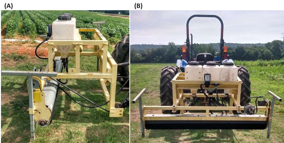
Fig. 1. Side (A) and rear (B) view of the two-row Grassworks® roller wiper used for both studies.
