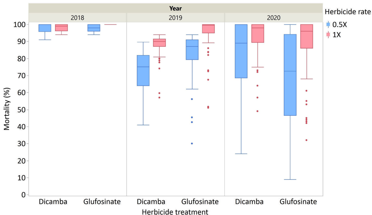
Fig. 2. Distribution of the annual mortality (%) of Palmer amaranth ( Amaranthus palmeri S. Wats.) accessions treated with dicamba or glufosinate at 0.5 or 1X rates (blue and pink boxes, respectively). Boxes represent 50% quartile, the line is the median value, and the points represent the outliers. Evaluations treated with 0.5X rate consisted of 52 and 71 accessions from 2018, 68 and 67 accessions from 2019, and 73 and 72 accessions from 2020 sprayed with dicamba and glufosinate, respectively. Evaluations treated with 1X rate consisted of 59 and 72 accessions from 2018, 62 and 66 accessions from 2019, and 85 and 77 accessions from 2020 sprayed with dicamba or glufosinate, respectively.
