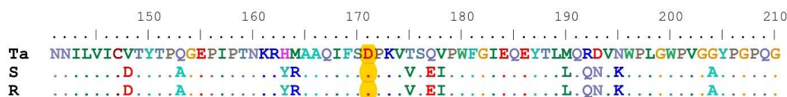
Fig. 1. Partial alignment of the glutamine synthetase gene of T. aestivum (Ta), glufosinate-susceptible (S), and glufosinate-resistant (R) accessions of Palmer amaranth. Yellow highlighting indicates amino acid position 171 based on the T. aestivum GS sequence (GenBank accession number: DQ124213.1).
