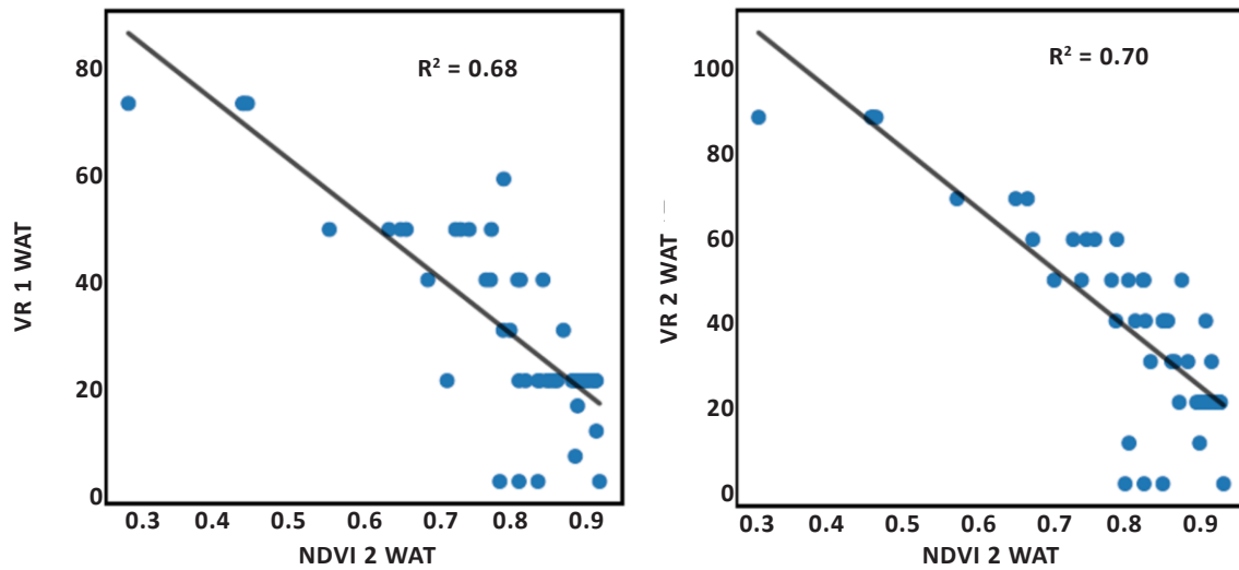
Fig. 7. Scatter plots with linear regression of normalized difference vegetative index (NDVI) 2 weeks after treatment (WAT) vs. visual estimations of injury (VR) 1 WAT (left) and 2 WAT (right) from plots receiving sublethal rates of auxin herbicide treatments on R2 soybean.
