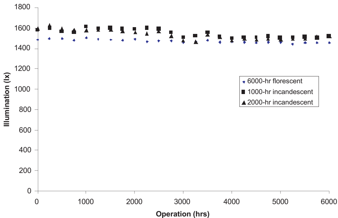
Fig. 2. Mean illuminance (lx) for the three types of lamps at 250-h measurement intervals
