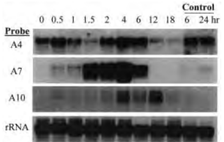
Fig. 3. Transcript accumulation in leaves following exposure to 1.0 µl (0.25 µM) of meJA. Leaves were collected at the time indicated, after intact plants were placed in a glass chamber for 1 hour with meJA. Membranes were hybridized with the indicated probes, and bands were visualized via autoradiography.
