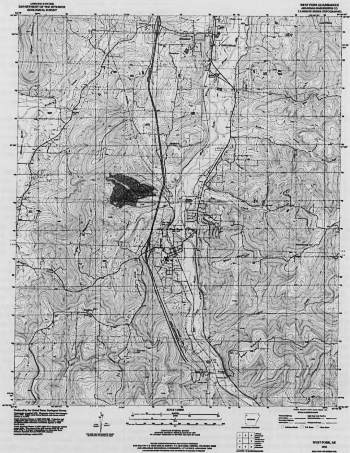
Fig. 3. United States Geological Survey 7.5-minute topographic quadrangle map of West Fork quadrangle, Washington County, Arkansas.
