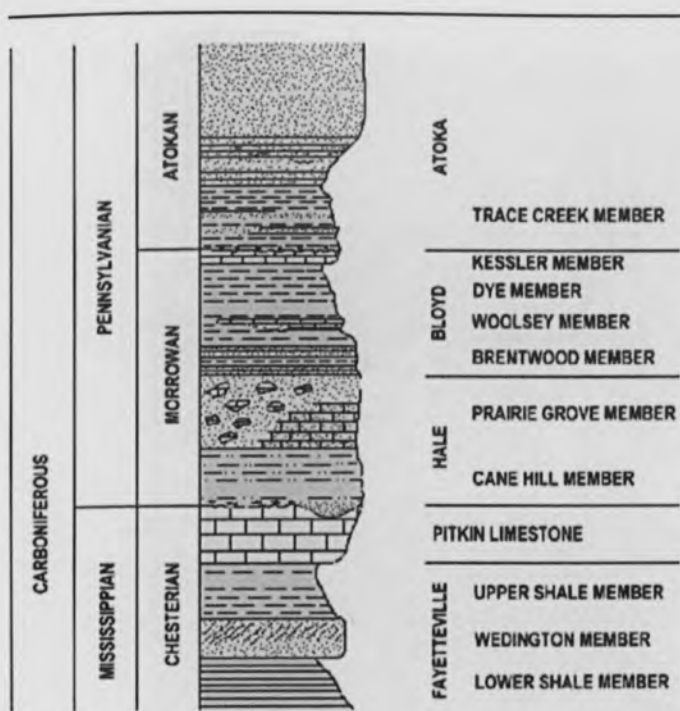
Fig. 2. Generalized stratigraphic column of West Fork quadrangle, Washington County, Arkansas (adapted from Brown, 2000; M.E. King, 2001).
