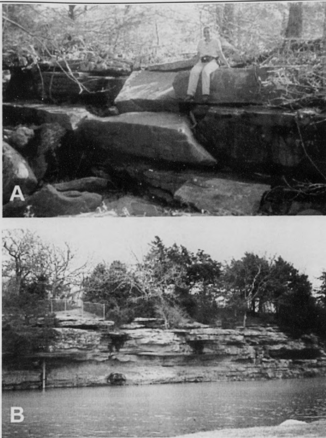
Fig. 7. A) The Wedington Sandstone Member of the Fayetteville Formation. This well-cemented sandstone commonly forms a bench of two meters in West Fork quadrangle. Located at UTM (WGS-84) Zone 15 S 396222 3983128. B) Thick section (approximately 10 m) of the Wedington Sandstone Member of the Fayetteville Formation exposed in a park along the West Fork of the White River in the community of West Fork, Arkansas at UTM (WGS-84) Zone 15 S 393223 3976680).
