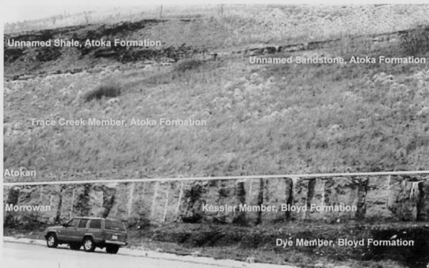
Fig. 12. Bloyd Formation – Atoka Formation contact. Road cut on the west side of Interstate Highway 540 shows the contact of the Kessler Limestone Member (Bloyd Formation) and Trace Creek Member (Atoka Formation) representing the Morrowan-Atokan. Location UTM (WGS-84) Zone 15 S 392505 3973721.
