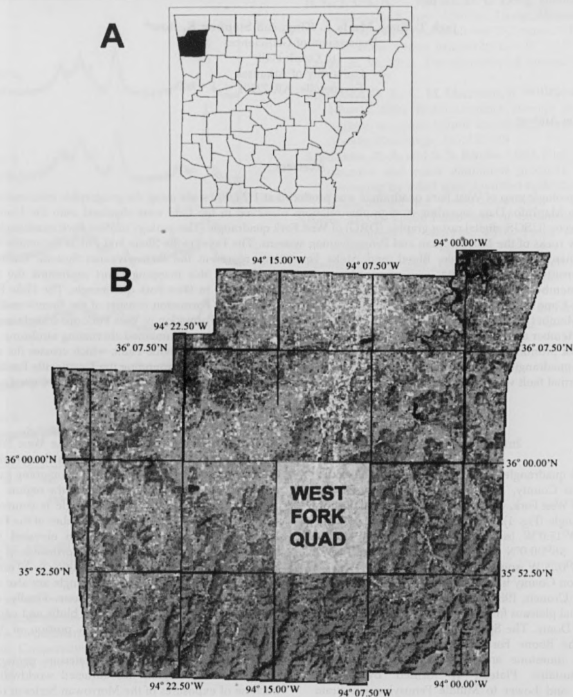
Fig. 1. A) Location map of Arkansas showing Washington County (shaded) and B) West Fork quadrangle in Washington County.
