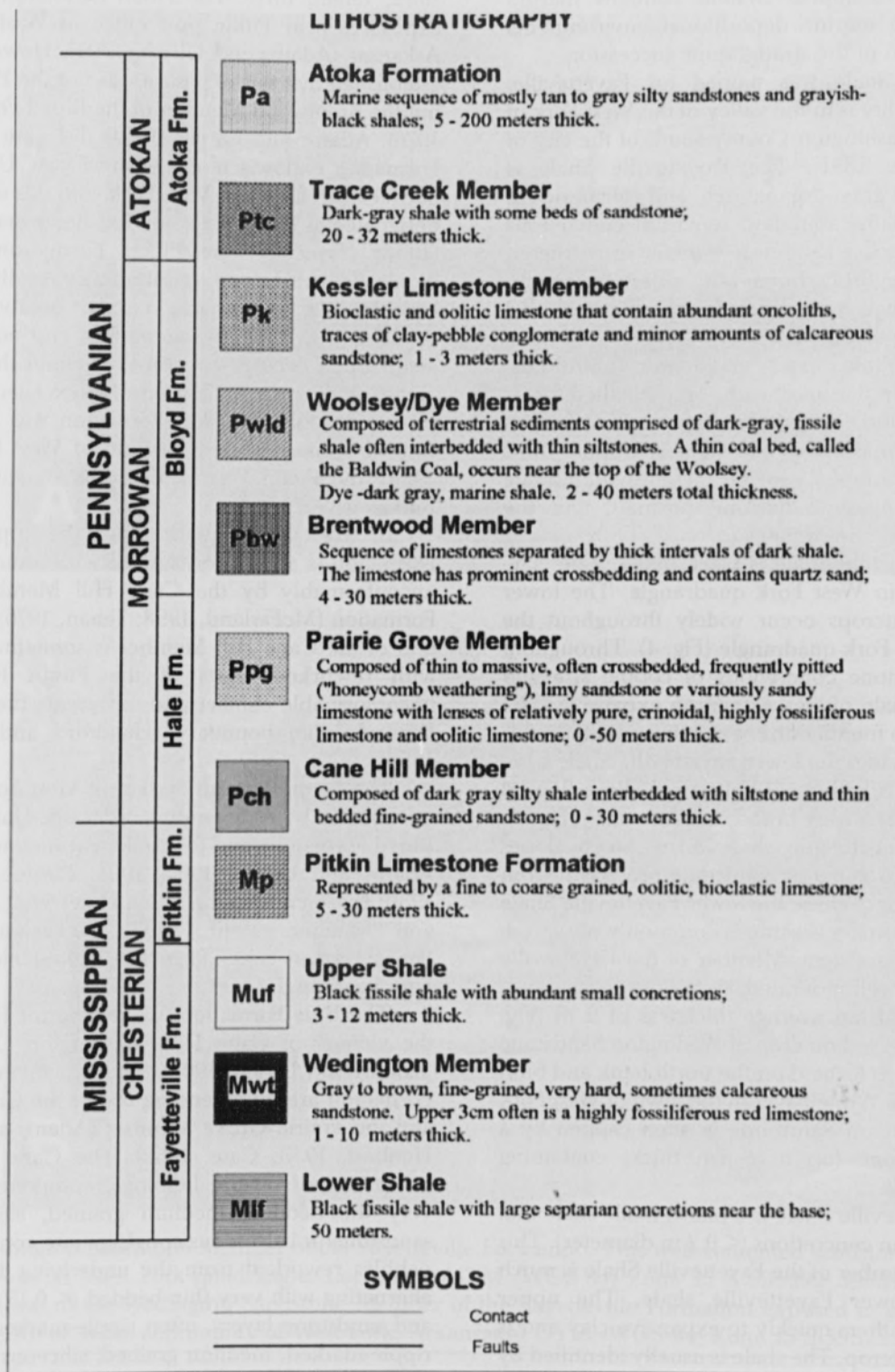
Fig. 6. Legend to accompany geologic map of West Fork quadrangle (Figs. 4 and 5).
