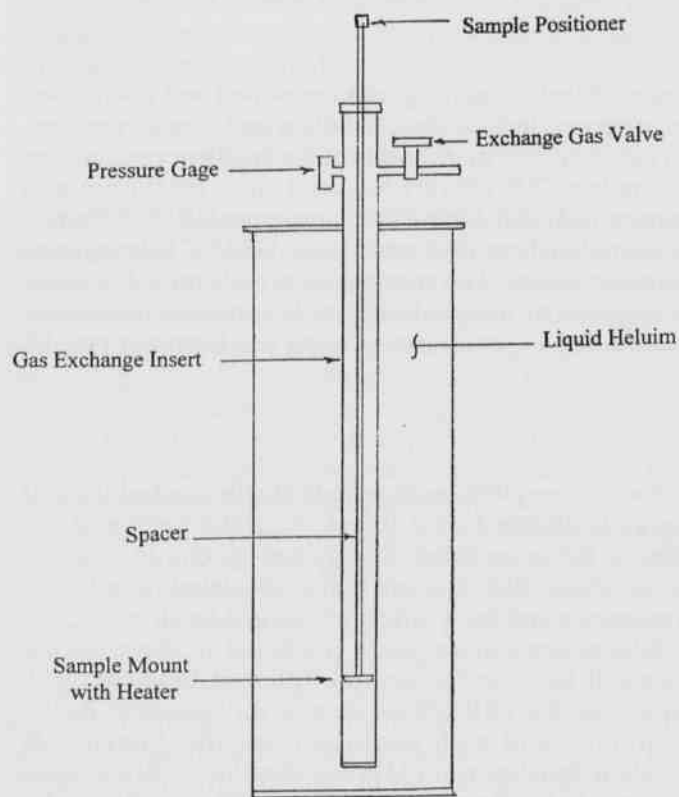
Fig. 3. Gas Exchange Insert for Cryostat
