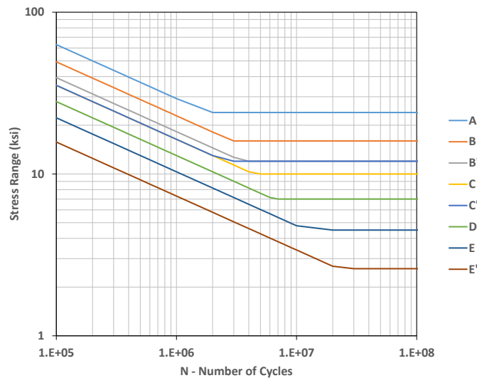
Figure 2-1: S-N Curves for each detail category
