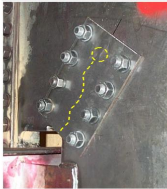
Figure 2-7: Splice Plate installed using high strength bolts (Dexter & Ocel, 2013)
