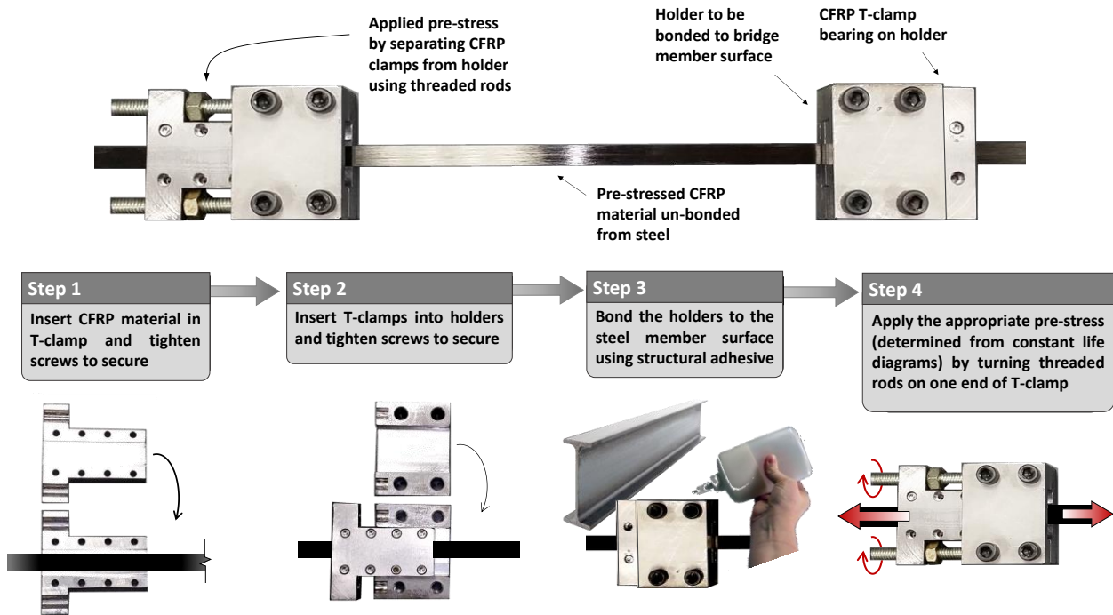
Figure 5-1: CFRP Retrofit and installation procedure
