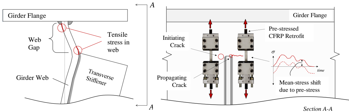
Figure 5-2: Example of retrofit installation on a partial depth web attachment showing shift in mean stress due to the pre-stressed CFRP.
