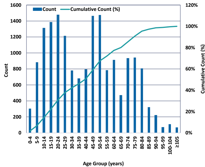
Figure 2-2: Age of Steel Highway Bridges in Region 6
