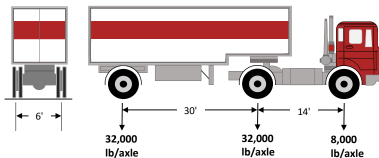
Figure 3-6: Characteristics of the AASHTO fatigue design truck HS 20-44
