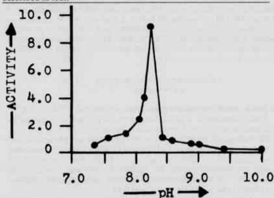
Figure 2. H. horridum venom phosphomonoesterase activity at various pH values. Activity is defined as the number of \mu\text{M} of p-nitrophenol liberated from p-nitrophenyl phosphate per min per mg of venom at 25°C.
