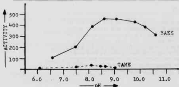
Figure 1. H. horridum venom arginine ester hydrolase activity with BAEE and TAME as substrates at various pH values of Tris • HCl (0.0667 M) buffer, 25°C. Activities were calculated by methods described in text.
