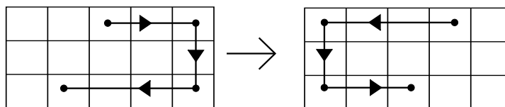
Figure 14: Cyclic Permutation
