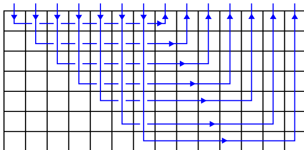
Figure 39: Here we have 7 nested strands on the n = 14 half-grid. This can be expanded for \frac{n}{2} nested strands on the n half-grid.
