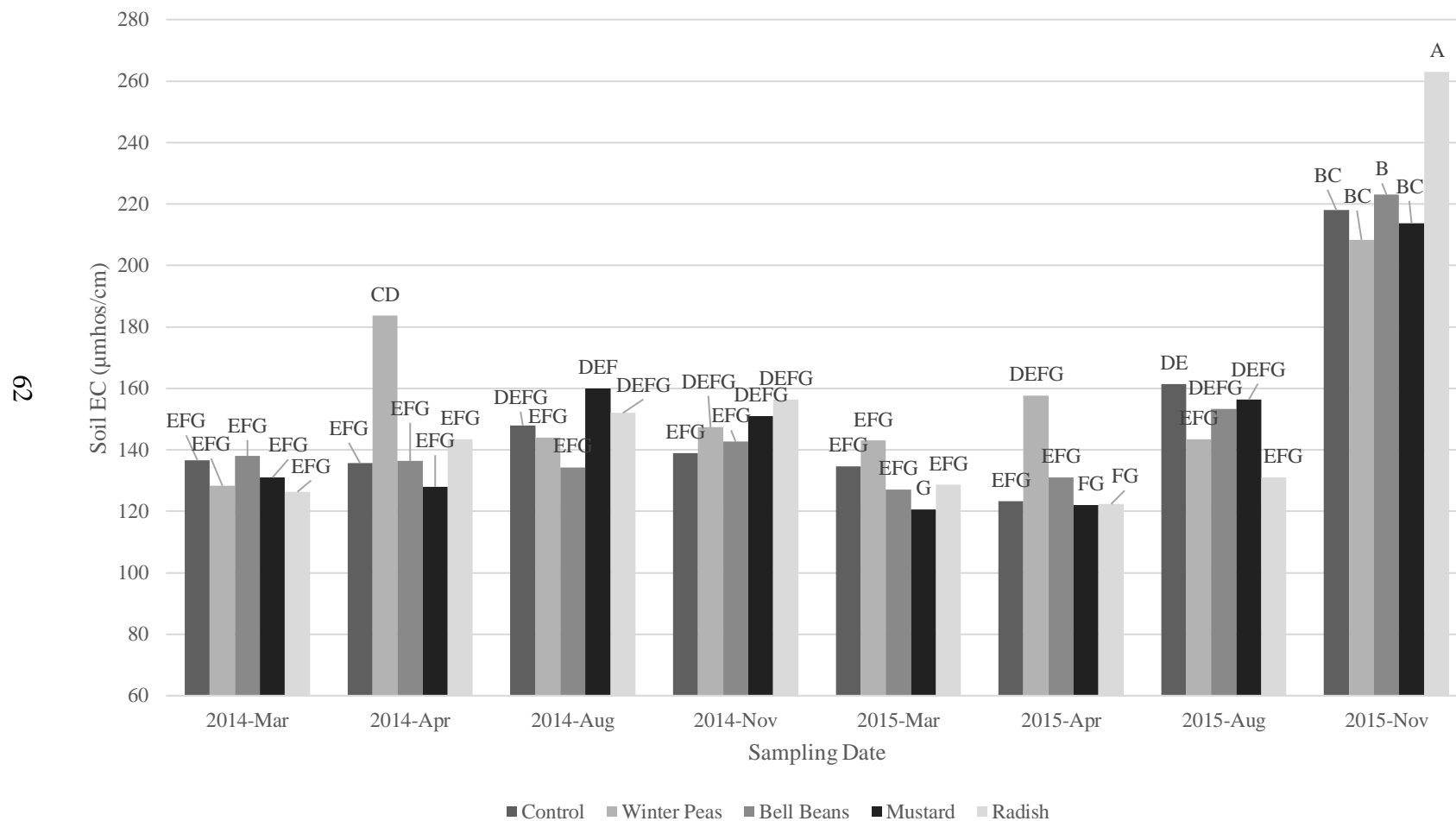
Figure 14. Soil EC ( \mu\text{mhos/cm} ) measured from 15 cm soil core samples collected on 28 Mar. 2014, 25 April 2014, 8 Aug. 2014, 7 Nov. 2014, 28 Mar. 2015, 28 April 2015, 12 Aug. 2015, and 12 Nov. 2015. March sampling dates are prior to cover crop incorporation, April dates are 30 days after incorporation, August dates are after tomato cropping, and November dates are after broccoli cropping in a high tunnel in Fayetteville, AR. Mean separation was performed by LSD at p < 0.05 . n = 3 experimental units.
