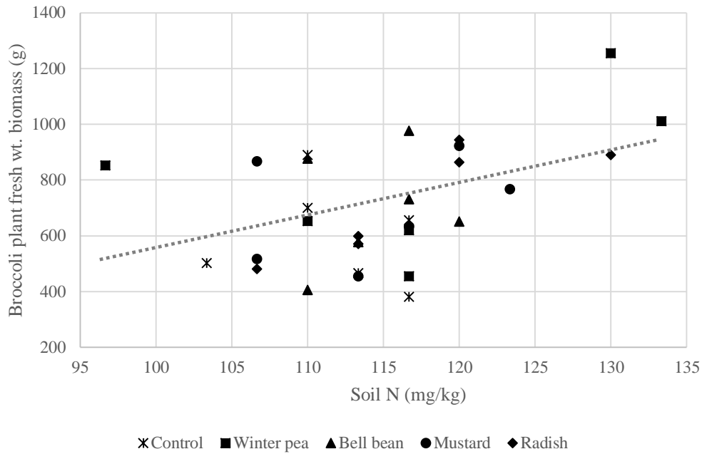
Figure 32. Relationship between soil N content and broccoli plant biomass, as measured from broccoli crops grown in a high tunnel in Fayetteville, AR. in 2014 and 2015. Soil N content was measured on 25 April 2014 and 28 April 2015, 30 days after the incorporation of cover crop treatments. Broccoli biomass was measured 7 Nov. 2014 and 9 Nov. 2015. Linear r^2 = 0.21 , n = 30 .
