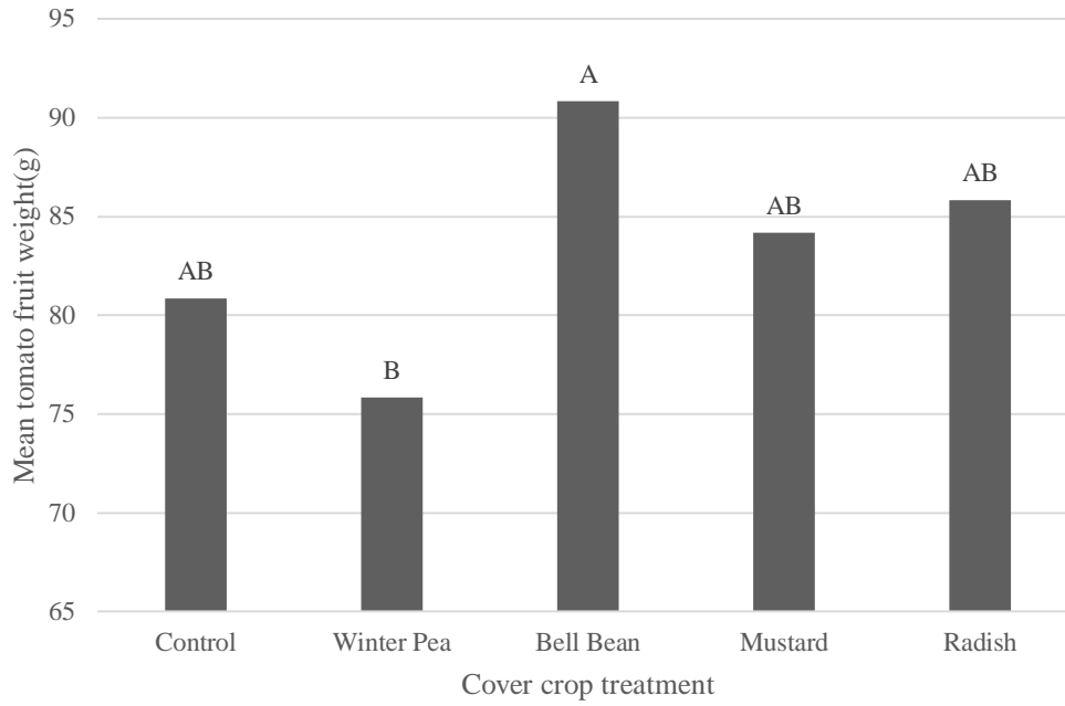
Figure 25. Tomato average fruit weight across years 2014 and 2015, measured from tomatoes grown in a high tunnel in Fayetteville, AR following winter cover crop treatments. Means comparison was conducted using Student's t test ( p < 0.10 , n = 3 ), with letters representing means separation.
