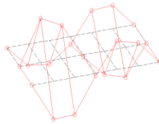
Butterfly Mode 2 f_8 = 87.875 Hz
