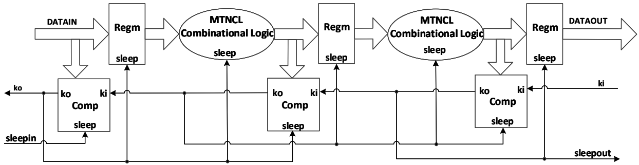
Figure 8: Multi-threshold NCL pipeline architecture.
