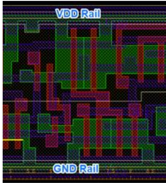
Figure 26: Power rails.
