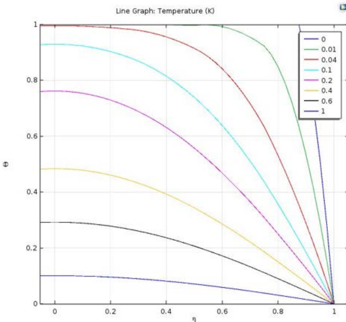
Figure 42. Temperature profile in a finite slab. The Legend shows dimensionless times.
