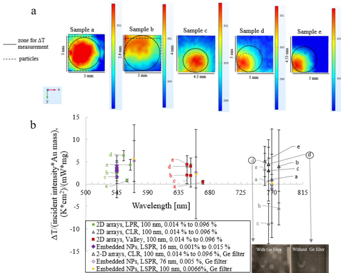
Figure 32. a) Experimental surface temperature plots (160 s heating) of Samples a-to-e at \lambda_{LPR} where particle zones and \Delta T calculation zones are enclosed with dashed and solid shapes respectively, b) Thermal responses of 2-D arrays across \lambda_{LPR} (filled green circles), \lambda_{valley} (filled red squares), and \lambda_{CLR} (filled grey triangles; open grey triangles with Ge filter) in comparison with random dispersions of 16 nm (filled violet diamonds), 76 nm (open violet diamond, Ge filter), and 100 nm (filled yellow diamond, Ge filter) NPs.
