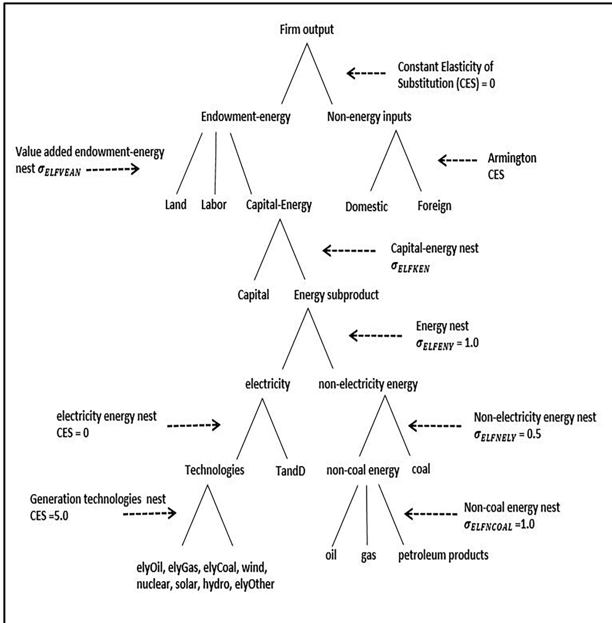
Figure 3-4 Modified GTAP-E production structure.
