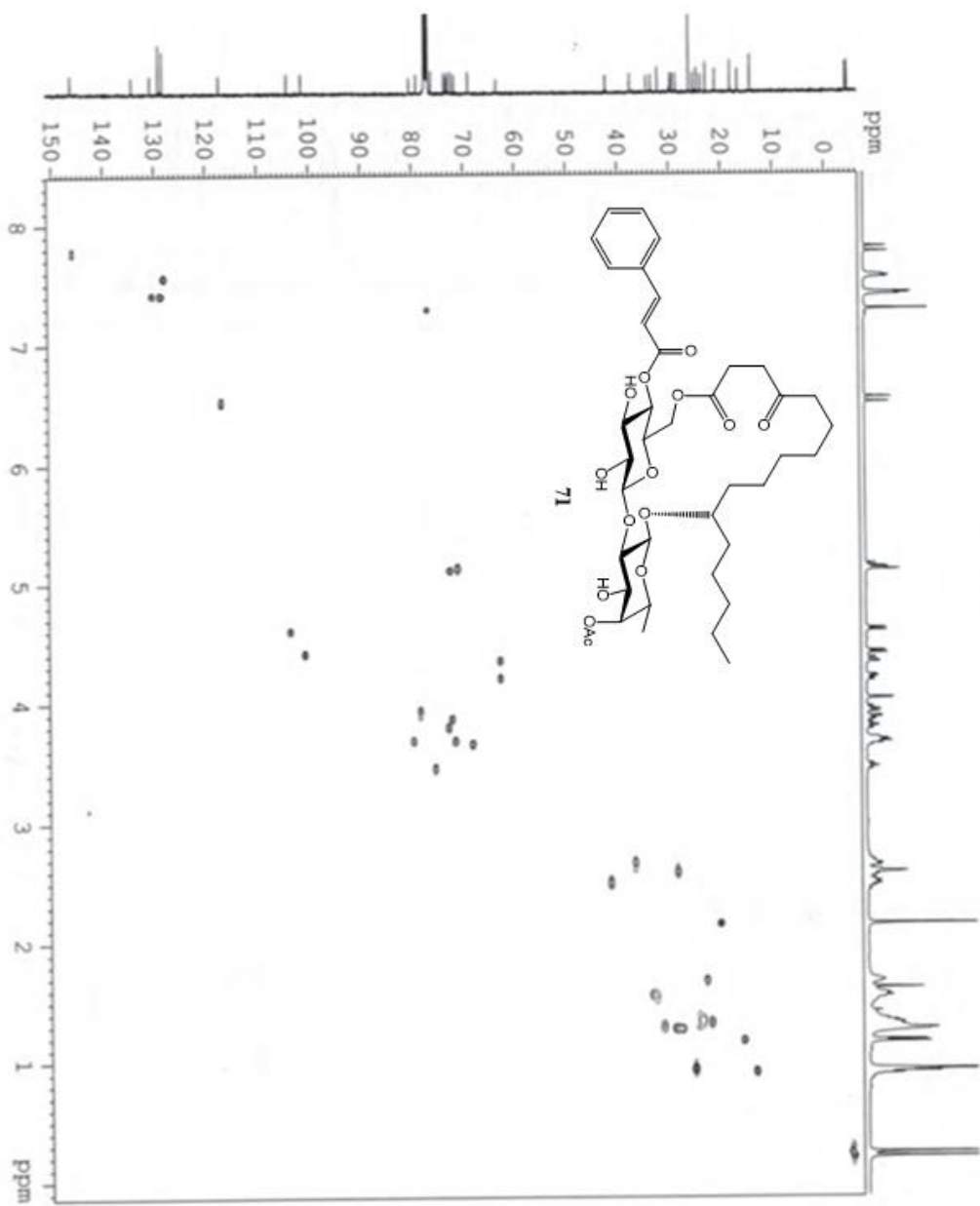
LW-1pomo-F-168- Product HSQC 400 LW
