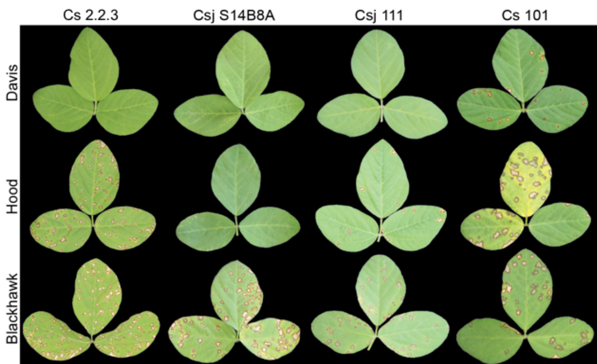
Fig 1. Summary of phenotypic reactions of C. soja isolates observed in this study. Soybean plants were inoculated with C. soja suspensions ( 1 - 3 \times 10^5 conidia/mL). C. soja 2.2.3 (Arkansas) isolate in which the new reference genome was assembled; Csj S14B8A (Illinois) represents the subcollection 1 (“Hood-avirulent”) while Csj 111 (Indiana) is a representative of subcollection 2 (“Hood-virulent”); Cs 101 (Arkansas) was one of the five isolates found to be virulent on cultivar Davis. Pictures were taken 14 days after inoculation.
