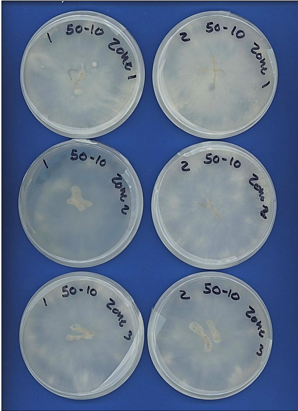
Figure 2-8. Examples of 'Rex' lettuce root isolations with Pythium grow out on PDA plates to confirm Pythium presence in roots. Root cuttings were taken from plants infected with Pythium myriotylum 'PM1'.
