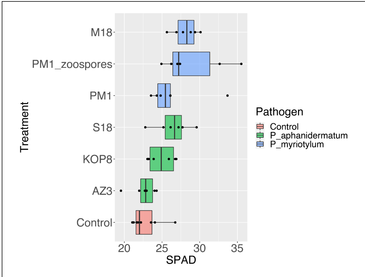
Figure 2-4. Effects of Pythium species and strain on hydroponic ‘Rex’ lettuce leaf SPAD chlorophyll content. Pythium species or control indicated by legend on the right where red color indicates the control, green color P. aphanidermatum , and blue color P. myriotylum . Pythium species and strains from top to bottom: P. myriotylum ‘M18’, P. myriotylum ‘PM1’ (oospores and zoospores), P. aphanidermatum ‘S18’, P. aphanidermatum ‘KOP8’, and P. aphanidermatum ‘AZ3’.
