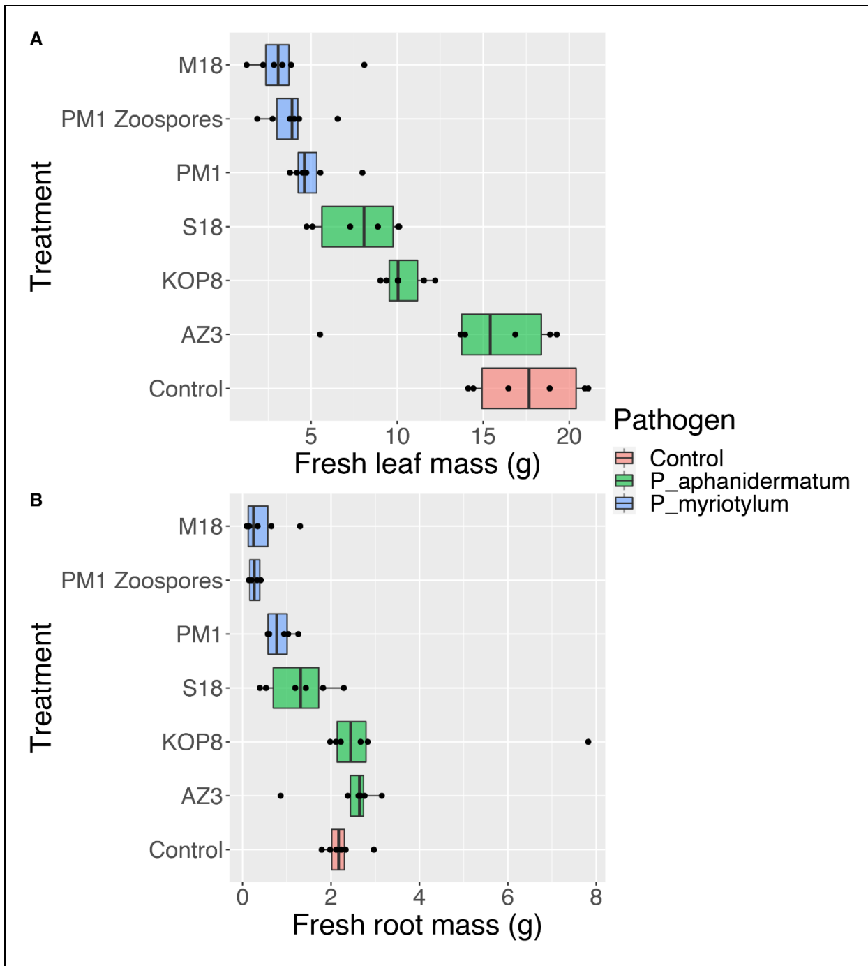
Figure 2-5. Effects of Pythium species and strain on hydroponic ‘Rex’ lettuce fresh leaf and root mass. Pythium species or control indicated by legend on the right where red color indicates the control, green color P. aphanidermatum , and blue color P. myriotylum . Pythium species and strains from top to bottom: P. myriotylum ‘M18’, P. myriotylum ‘PM1’ (oospores and zoospores), P. aphanidermatum ‘S18’, P. aphanidermatum ‘KOP8’, and P. aphanidermatum ‘AZ3’.
