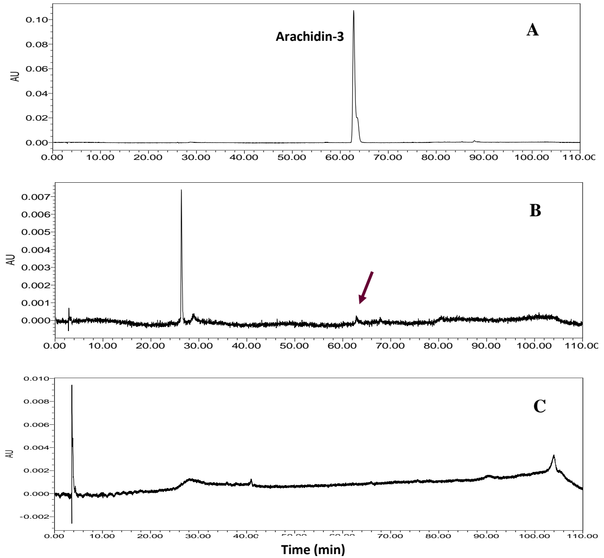
Figure 8. HPLC Chromatogram of (A) arachidin-3 standard, (B) apical sample treated with 100 \mu\text{M} of arachidin-3 and (C) basal sample treated with 100 \mu\text{M} of arachidin-3 at time point 2 hr.
